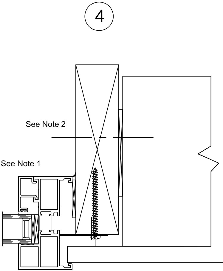
CONCRETE INSTALLATION
