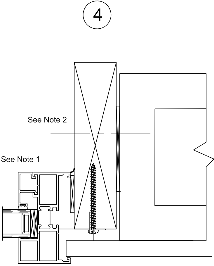
CMU INSTALLATION
