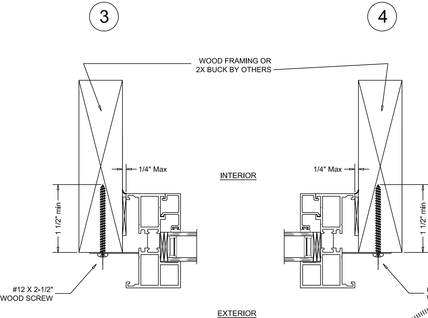
HORIZONTAL SECTION DETAIL WOOD FRAMING INSTALLATION
